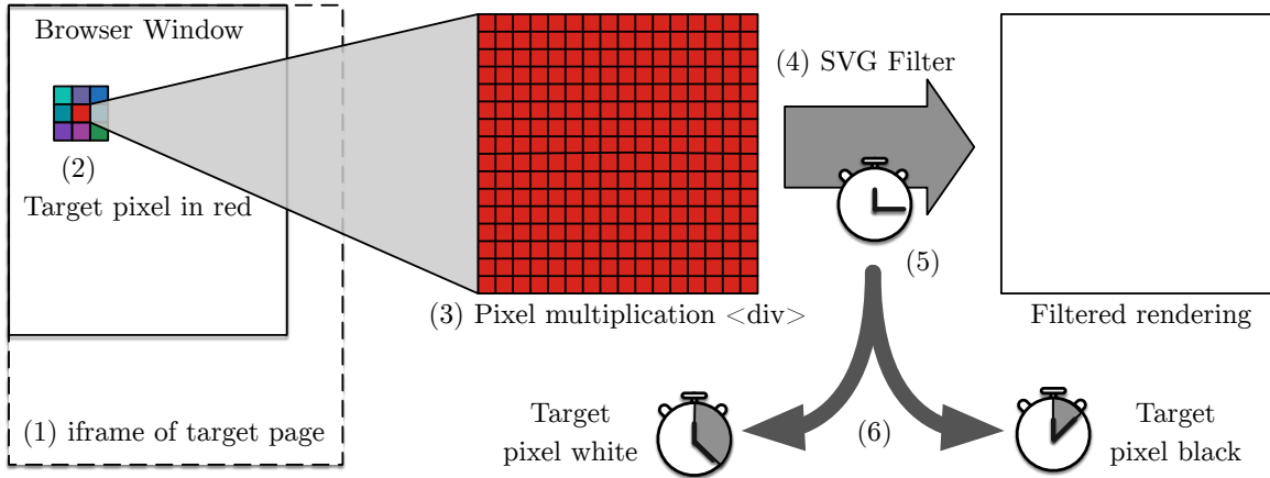
Figure 3: Cross-Origin SVG Filter Pixel Stealing Attack in Firefox, reproduced from [2] with permission
